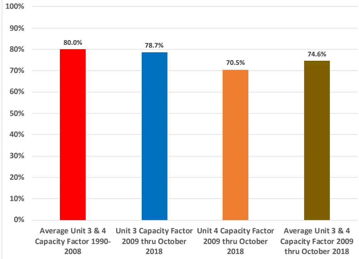
Figure 7: Colstrip Unit 3 and 4 Equivalent Availability Factors Before and After 2008 (EAF) 30
